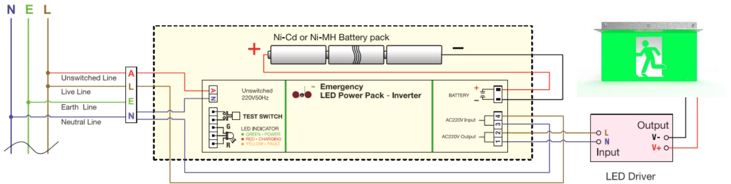
100% Output wiring diagram (Maintained Type)
